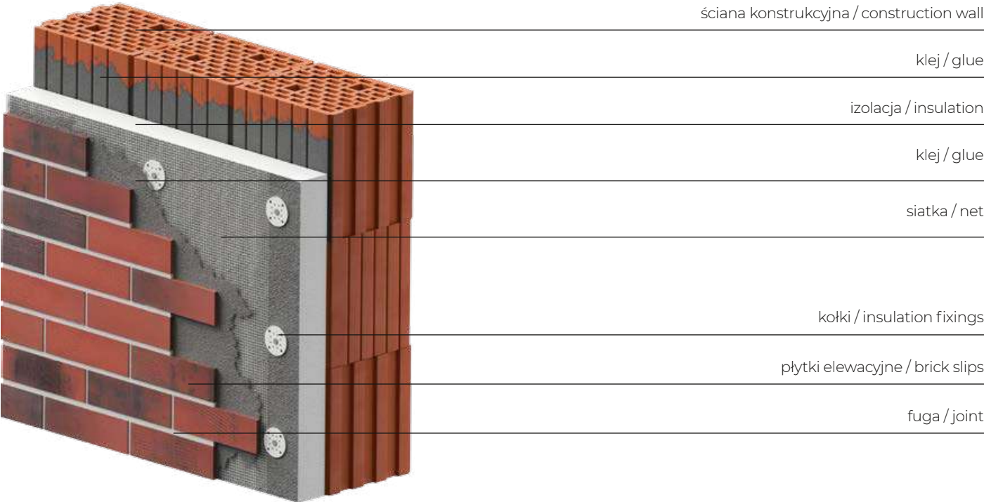
System dociepleń na styropianie eps / System of insulation on EPS foam
