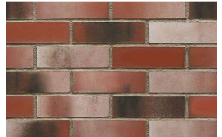
Supernova HF79
