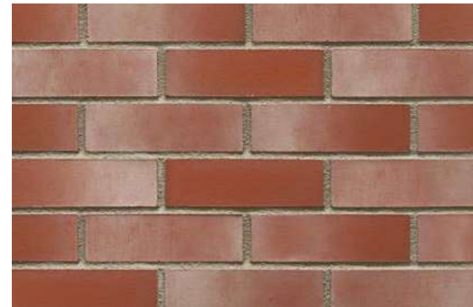
Stardust HF78
